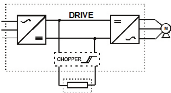
Circuit example
